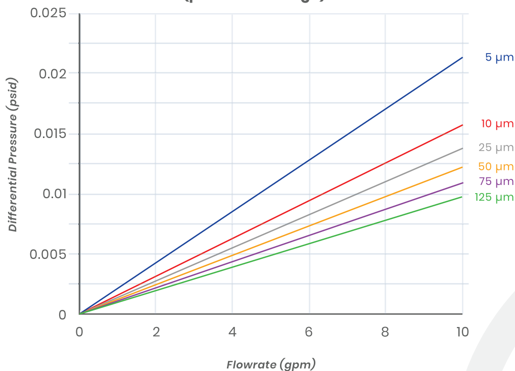
Typical Flow Rate Clean Water at Ambient Temperature (per 10" cartridge)
